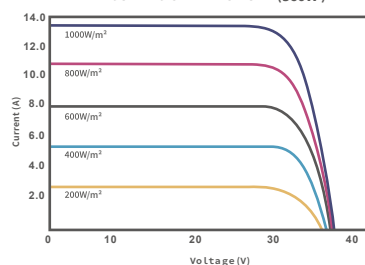
I-V CURVES OF PV MODULE (560W)
