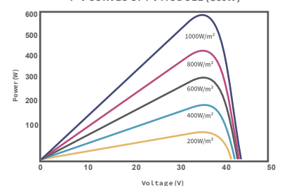
P-V CURVES OF PV MODULE (560W)
